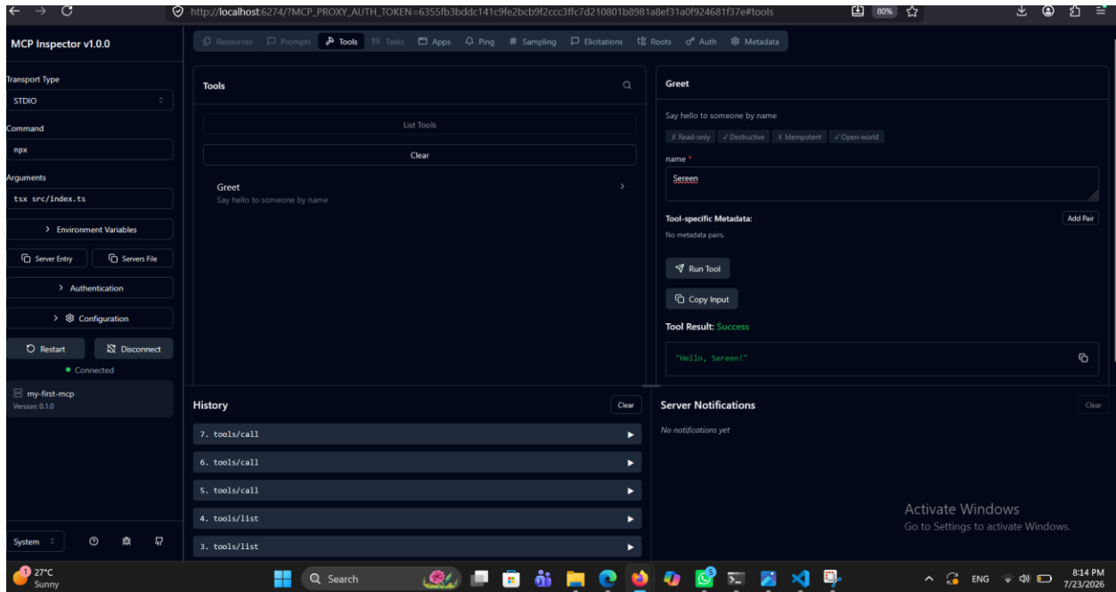
Figure 1: MCP Inspector connected to the server and successful execution of the greet tool.
